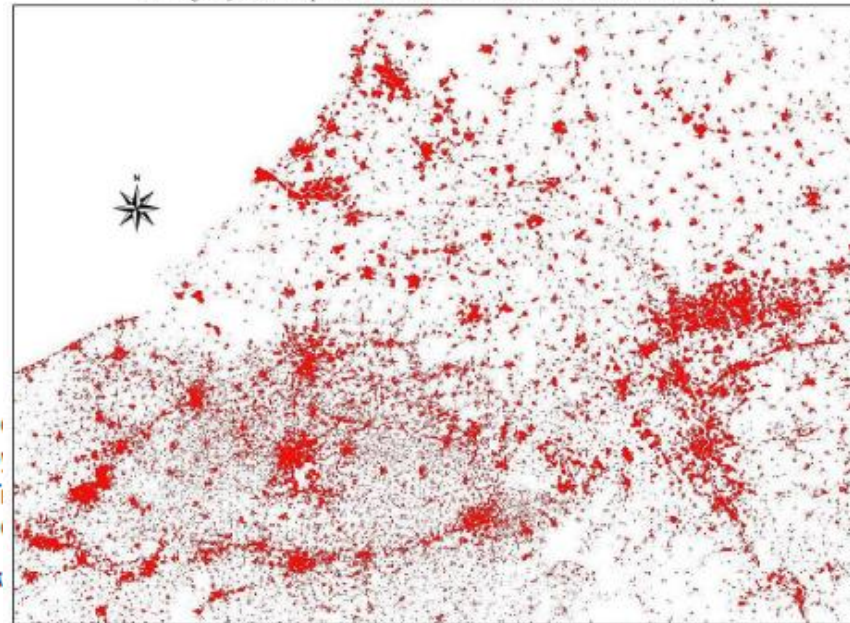
Heterogeneity of built-up areas at the level of North-Western continental Europe
